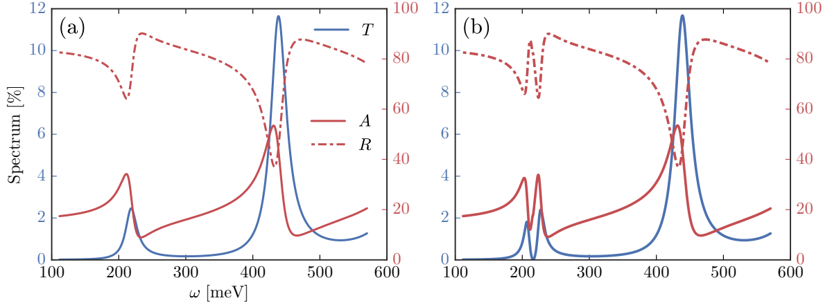
Figure 3.2: Transfer matrix transmission ( T ), reflectivity ( R ) and absorption ( A ) spectra for the (a) bare micro-cavity and (b) the resonator filled with PVAc molecules. Calculations are obtained via the open source library tmm in Python [292].
