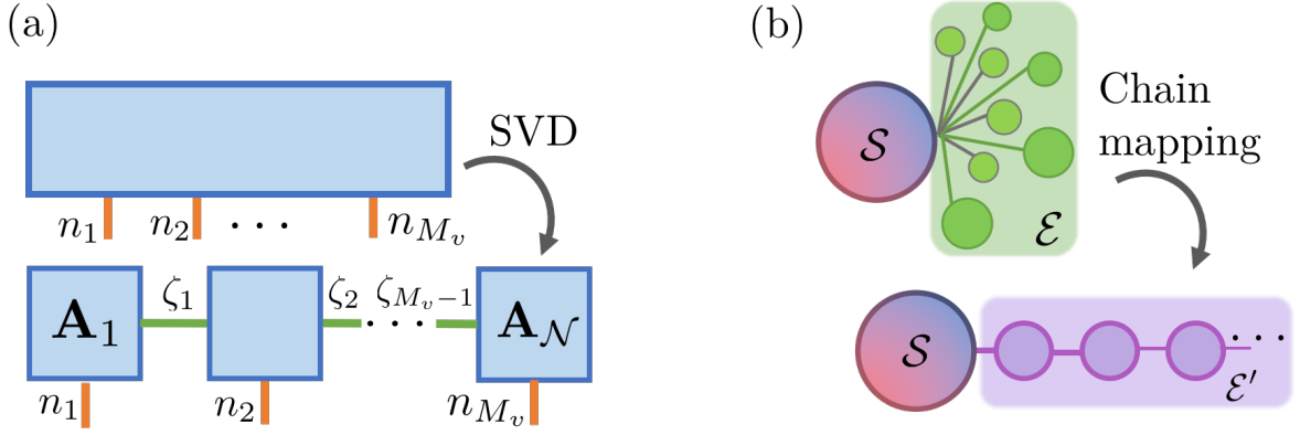
Figure 2.3: (a) Sketch of the ‘breaking’ by repeated SVDs of the system wavefunction into tensors connected by virtual bonds. The representation of the bath in an optimal boson basis is also displayed. (b) Mapping of the system-environment Hamiltonian into a 1D lattice or chain, where operators act on local Hilbert spaces where each \mathbf{A}_k is defined.
