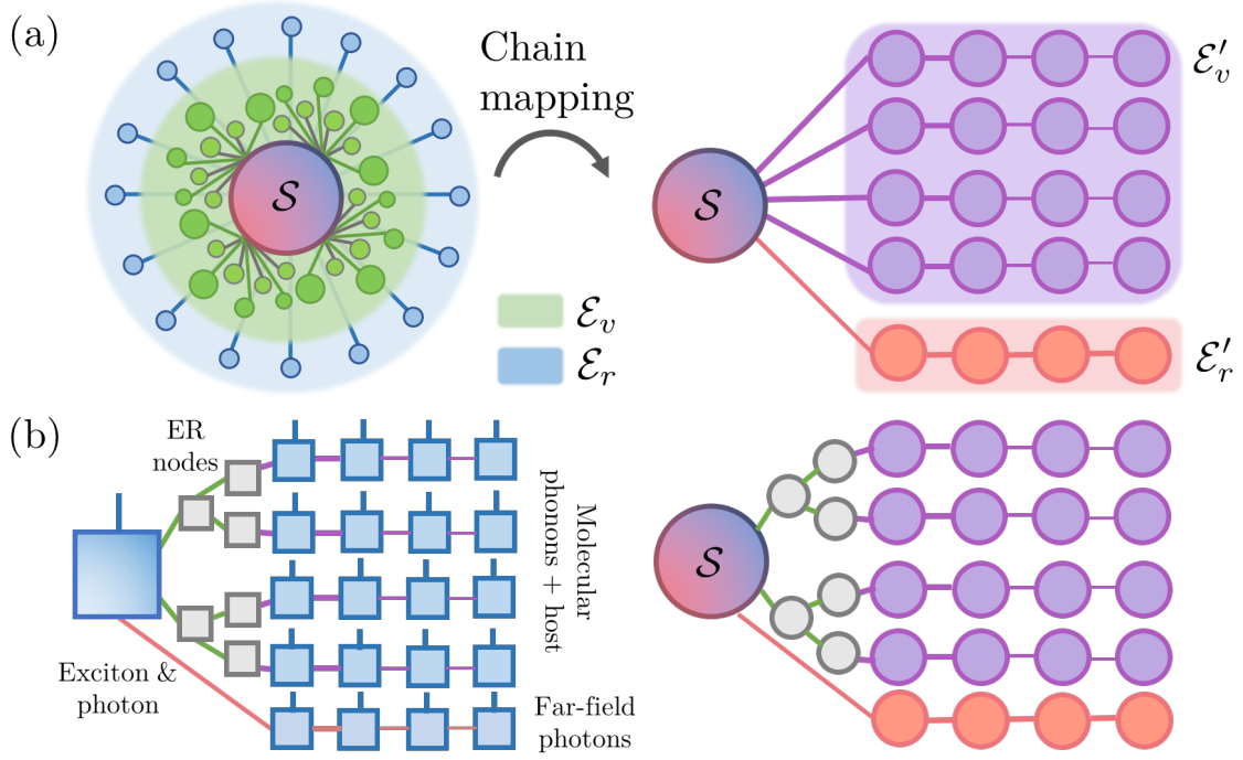
Figure 2.4: (a) Chain mapping of the multi-environment Hamiltonian in text to a star-structure that includes excitonic and photonic degrees of freedom in the root operator. (b) Efficient representation as a TN by further SVDs of the root node in the star-TN to form a tree-like structure introducing auxiliary non-physical sites (left) and corresponding coupling structure in the Hamiltonian.
