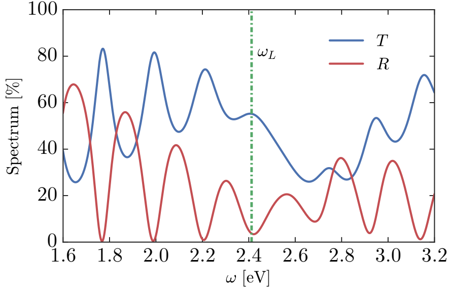
Figure 4.4: Transmission and reflection spectrum for the cavity used in Shalabney et al VSC experiment in the visible region (10 nm— Au mirror -2\ \mu\text{m} PVAc -10 nm Au mirror). The dielectric functions employed for the gold mirrors and the molecular layer are introduced in section 3.2 .
