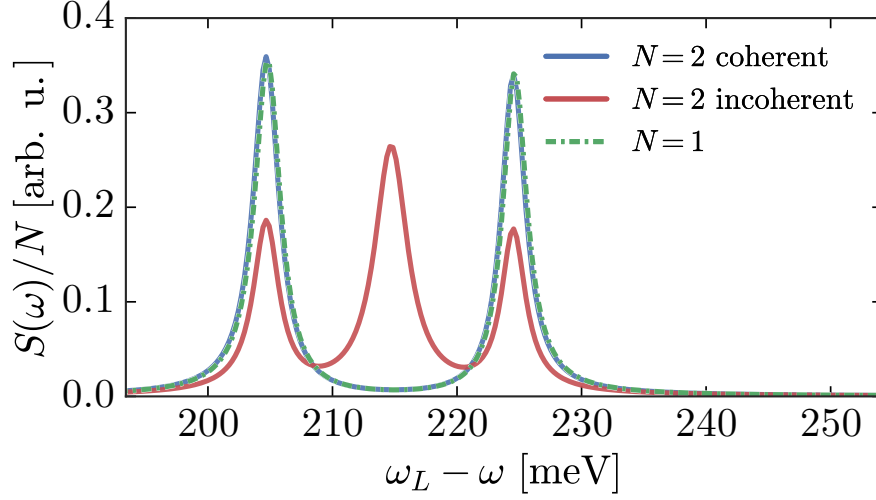
Figure 4.3: First Stokes line of the Raman spectra in the strong coupling regime, for one and two molecules. The chosen parameters are the same as those used for the single-molecule case, with the spectra normalised to the number of molecules N . For the case of two molecules, the spectra for coherent and incoherent collection are depicted. For comparison, the case of a single molecule already shown in Figure 4.2b is also rendered.
