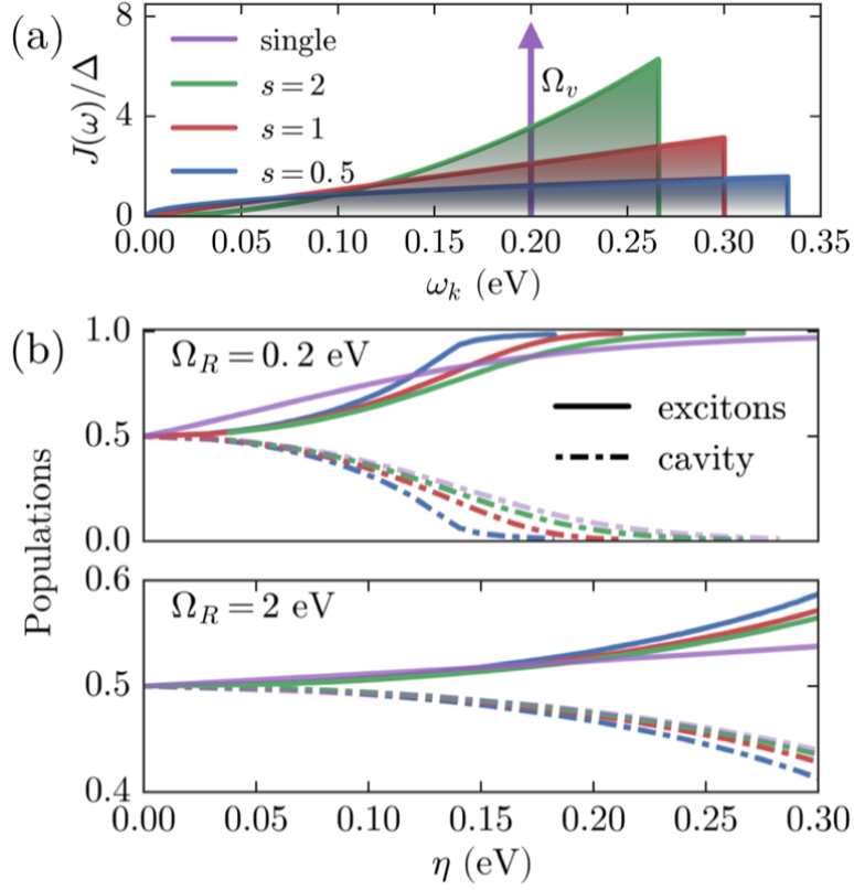
Figure 6.4: (a) Functional forms adopted for the LPP calculation and (b) Reduced populations over subsystem \mathcal{S} in the LPP as a function of the coupling strength to the reaction coordinate \eta . Here different curves correspond to the different spectral densities in (a), depicting in the upper and lower windows of (b) the cases for Rabi frequency shown.
