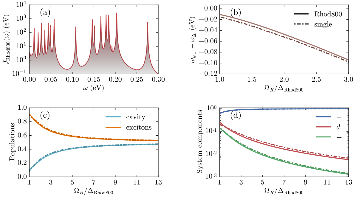
Figure 6.10: Reduced observables for the LPP supported by a dimer of Rhod800 molecules. The total reorganisation energy for the modes that are considered is \Delta = 112 meV. The numerical first moment of the spectral density J_{\text{Rhod800}}(\omega) , depicted in panel (a) reveals a value of \Omega_v = 154 meV.
