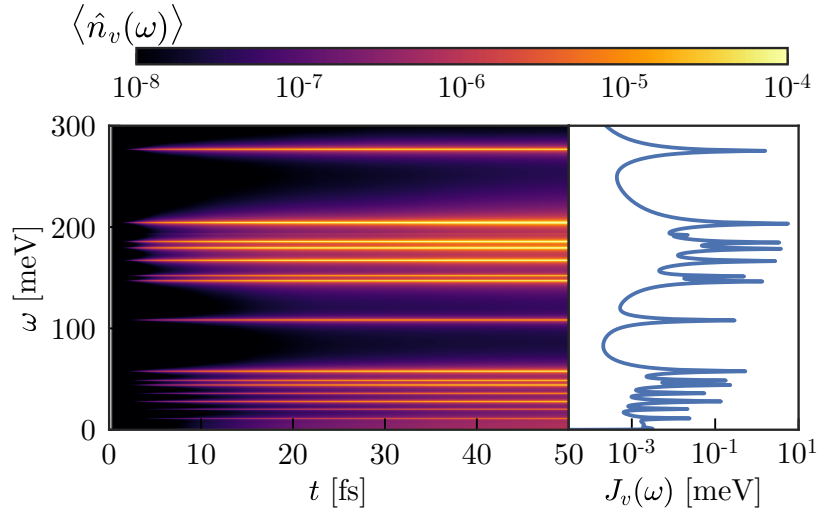
Figure 7.3: (left) Dynamics of the phononic mode populations for a single molecule for a fixed Rabi frequency \Omega_R = 0.1 eV and (right) sketch of the spectral density considered.
