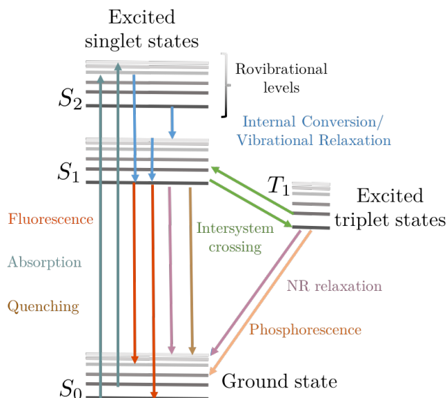
Figure 1.3: Jablonski diagram displaying transition processes that occur triggered by external excitation. The colours for the arrows and labels for each process are matched. Electronic states are denoted by their total spin. Only a portion of the rovibrational states is represented due to their massive number of typical molecules.
