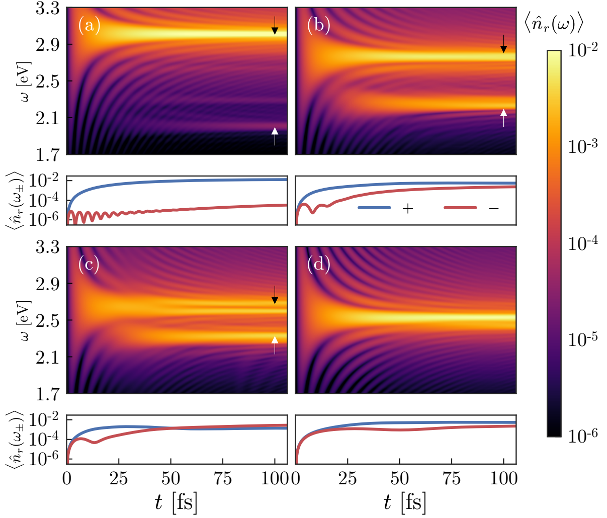
Figure 7.5: Far-field photonic population as a function of frequency and time, for the same Rabi splittings as in Figure 7.4 and N = 4 . The black and white arrows in panel (a-c) point to the approximate location of the bare UP and LP. Each panel includes in the lower parts cuts at \omega_{\pm} .
