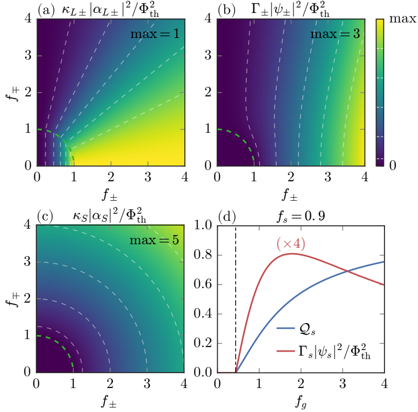
Figure 5.3: Rescaled population densities under two-mode pumping with \Phi_{\text{th}}^+ = \Phi_{\text{th}}^- , for (a) the pump mode, (b) the polaritons and (c) the Stokes mode. The green dashed semicircles denote the threshold condition f_{\text{tot}} \geq 1 . (d) Quantum efficiency \mathcal{Q}_S (blue) and rescaled signal polariton density (red, multiplied by 4 for clarity) at a signal pump strength of f_s = 0.9 as a function of the gate pump strength f_g .
