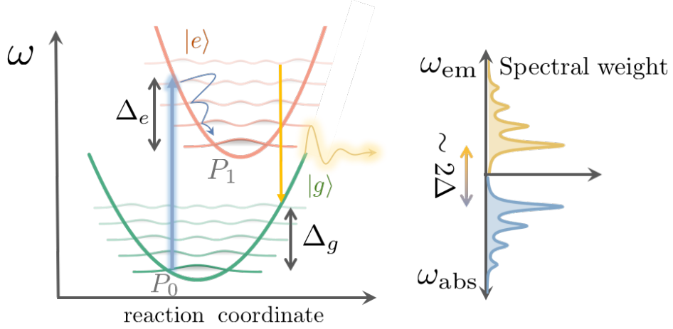
Figure 2.2: (a) Sketch of optical absorption and emission processes in the Franck-Condon limit (b) Typical steady-state absorption and emission spectra associated to this dynamics.
