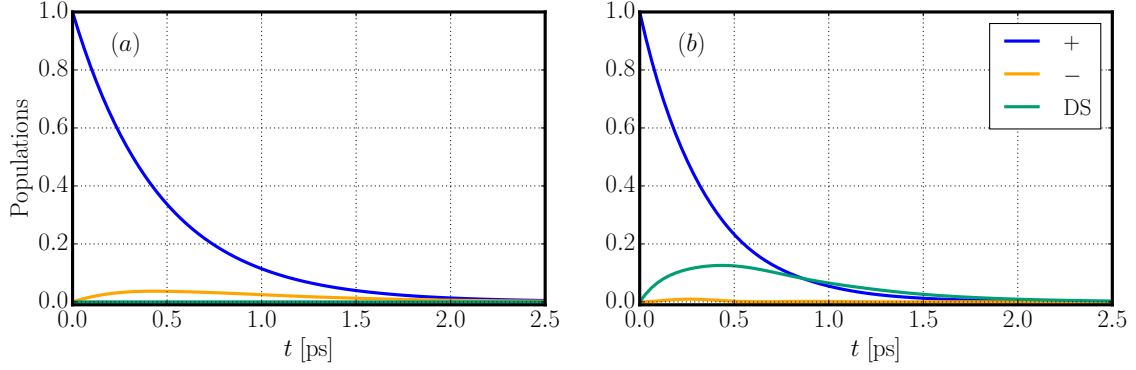
Figure 3.5: Population dynamics starting from the initially excited upper polariton |+\rangle for the two possible dephasing scenarios: (a) Common bath and (b) independent baths. The parameters are the same as in Figure 3.4b, with f = 0.5 and N = 100 . Each panel shows the upper and lower polariton ( \pm ) populations, as well as the total population in all dark states (DS), given by \text{Tr}(\hat{\mathcal{P}}_{\mathcal{D}}\hat{\rho}) .
