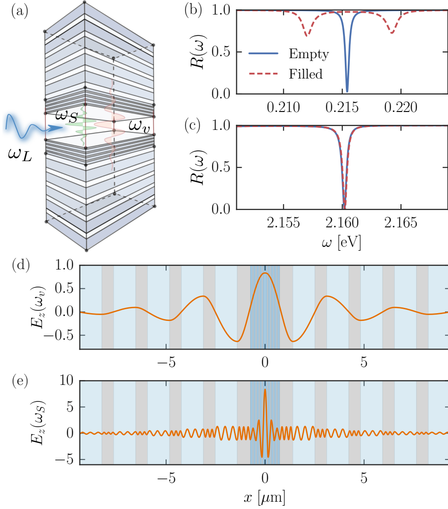
Figure 5.2: (a) Sketch of a double DBR cavity for both mid-IR and optical modes (not to scale). The blue arrow depicts the driving beam, while the green and red fields sketch the confined modes. (b,c) Reflectivity spectra in the mid-IR and visible region. The doublet in (b) is a signature of VSC with the C=O bond stretching mode of PVAc at \omega_v = 215 meV. (d,e) Cavity structure and electric field profiles (in arbitrary units) of the mid-IR and optical cavity modes. The DBRs consist of SiC (grey), SiO 2 (light blue), and PVAc (medium blue).
