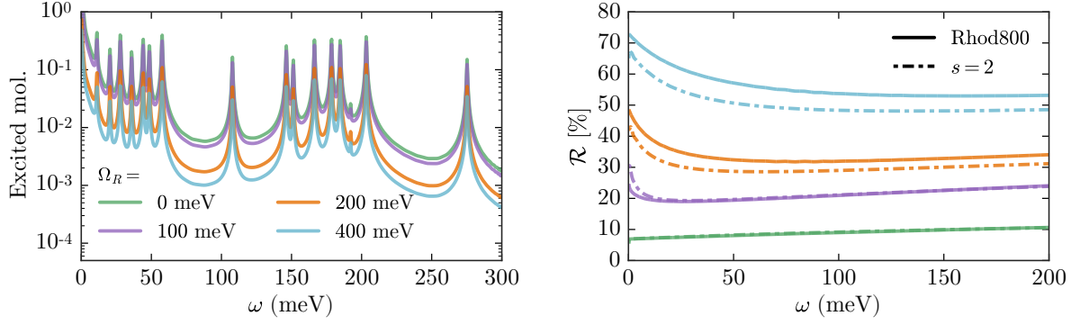
Figure 6.11: (a) Displacement spectrum for the LPP supported by a dimer of Rhod800 molecules, projected on the electronically excited molecule. (b) Ratio between the displacement of the electronically excited molecule at \Omega'_R = 1.5 eV and the cases depicted in (a). The remaining parameters are fixed according to Figure 6.10 caption.
