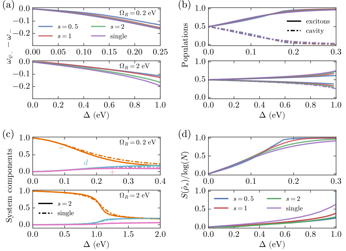
Figure 6.5: (a) Energy shift with respect to the bare lower polaritons ( \Delta = 0 ), (b) exciton/photon fractions (c), vibration-free components in the LPP and (d) Von-Neumann entropy of the photonic-excitonic and vibrational states bipartition, as a function of reorganisation energy. In these panels upper panels depict the case \Omega_R = \Omega_v and \Omega_R = 10\Omega_v = 2 eV for the lower panels.
