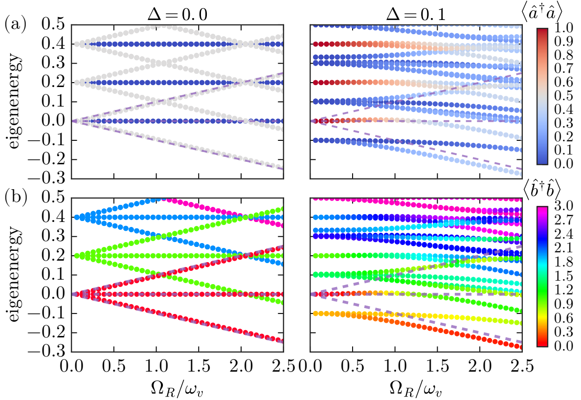
Figure 6.3: (a) Photonic components in the eigenspectrum of the HTC model for two molecules as a function of the ratio between Rabi frequency \Omega_R and vibrational frequency \omega_v . (b) Total vibrational components, \langle \hat{b}^\dagger \hat{b} \rangle = \sum_i \langle \hat{b}_i^\dagger \hat{b}_i \rangle . Dashed purple lines indicate the upper and lower vibration-free polariton and excitonic dark state energies. Similarly, \omega_e = \omega_O = 0 .
