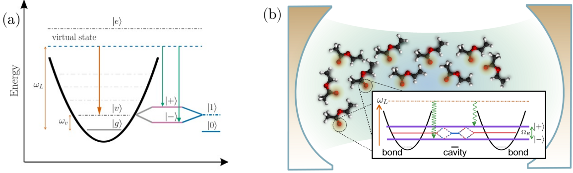
Figure 4.1: (a) Sketch of the RS process for a molecule as a result of excitation with an off-resonant driving field. After coherent excitation, the molecule promotes to a virtual state depicted with a blue dashed line. In the weak coupling regime, the electron decays into the first excited vibrational state, |v\rangle (orange arrow). When this first excited vibrational state is strongly coupled to the cavity mode, |1\rangle , the electron can decay to any of the two polaritons, |+\rangle or |-\rangle (blue arrows). (b) Sketch of mid-IR illustrating the Raman effect into delocalised polariton states.
