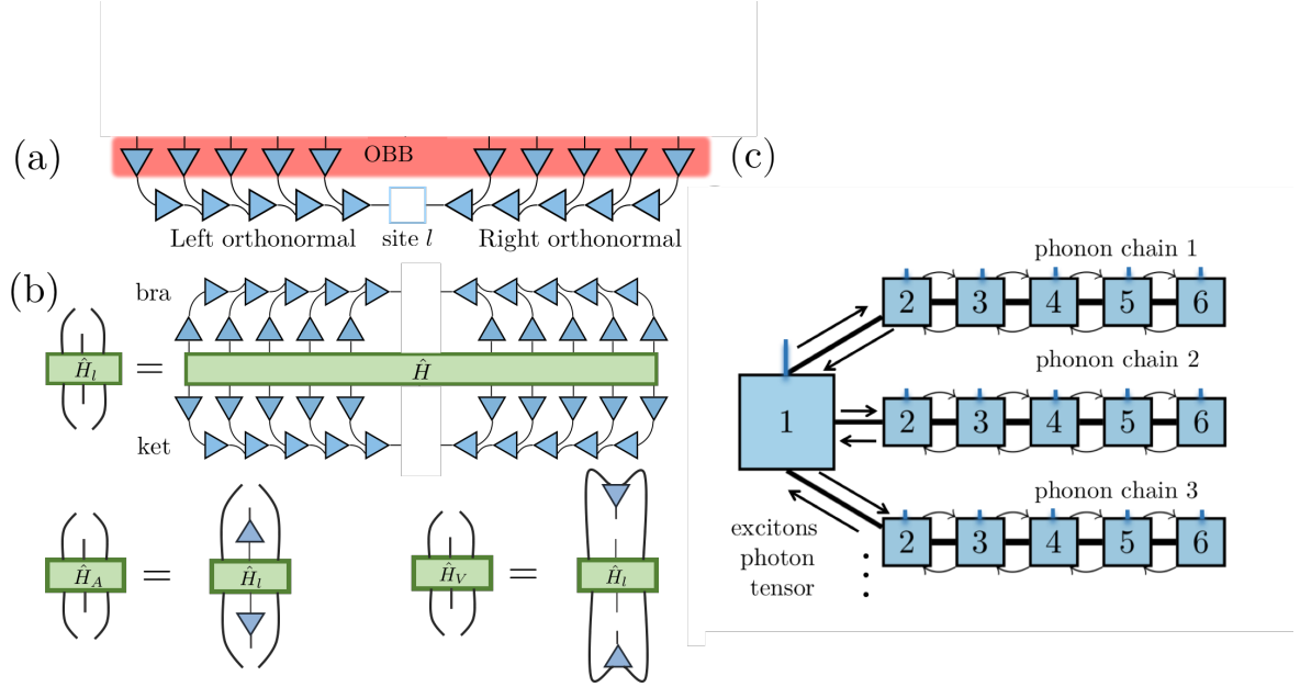
Figure 2.5: (a) Mixed canonical representation of a one-dimensional MPS, focused on site l , where the triangle orientation indicate the normalisation conditions, with the notation employed in [194, 195] and (b) effective one-site Hamiltonians that are instrumental to perform efficiently the variational optimisation of the all different types of tensors in the TN. (c) Sketch of the DRMG sweep procedure for the star-TN TN for the case N = 3, M_v = 5 that is used to represent the variational wavefunction in Equation 2.50.
