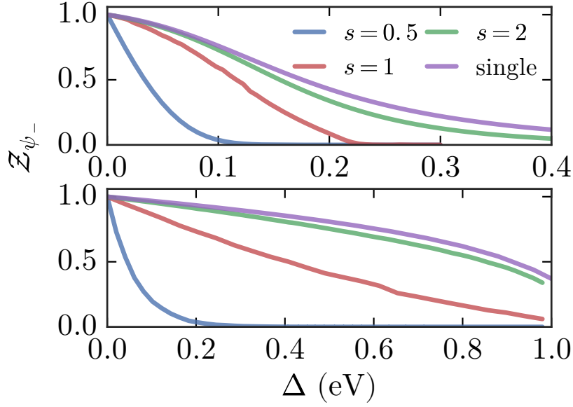
Figure 6.7: Overlap of the LPP wavefunction with the vibration-free polariton |-\rangle for \Omega_R = 0.2 eV (upper panel) and \Omega_R = 2 eV (lower panel) for the HTC and J_v(\omega) in the form Equation 6.3.
