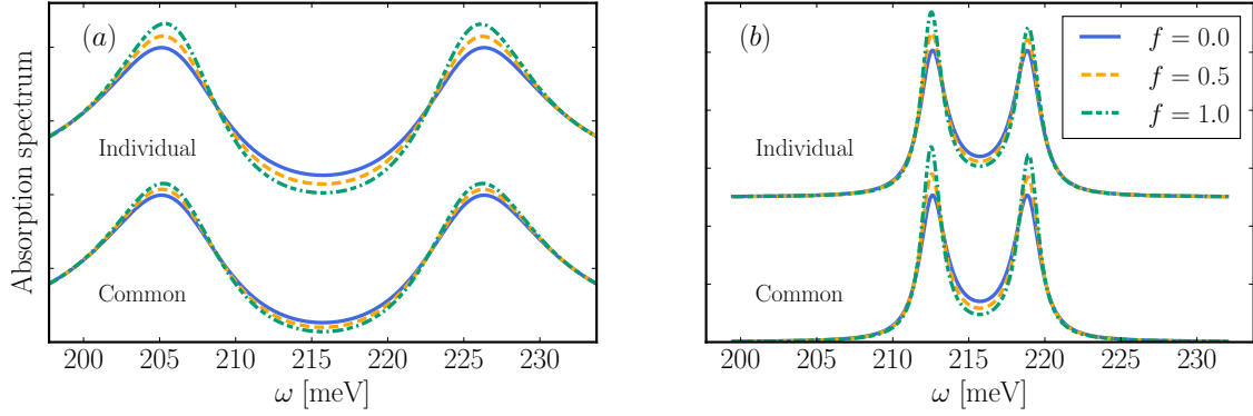
Figure 3.4: Absorption spectra for the two possible dephasing scenarios as a function of f . In both panels the two sets of curves are offset for a better visualization. In panel (a), the parameters used for the calculations are those reported in Ref. [140] (see text), whereas in panel (b), the Rabi splitting and the cavity decay rate are reduced to \Omega_R = 6.5 meV and \kappa = 1 meV, respectively.
