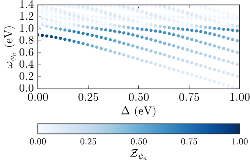
Figure 6.6: Excitation spectrum |\psi_n\rangle of \hat{H}_S + \hat{H}_v for a HTC model with N = 2 molecules and \Omega_R = 0.2 eV. The color-scale indicates the overlap with the bare lower polariton \mathcal{Z}_{\psi_n} with increasing saturation.
