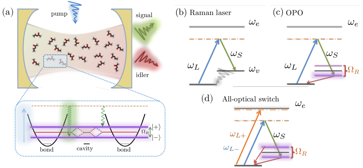
Figure 5.1: (a) Sketch of setup to convert a Raman laser into an OPO through vibrational strong coupling. The lower part of the figure shows the hybridisation between molecular bonds and the infrared cavity mode schematically. (b) In a Raman laser, Raman scattering of the pump (blue arrows) leads to vibrationally excited final states that decay non-radiatively, so that only a signal beam (green) is emitted. (c) Under strong coupling of the vibrational excitations with a resonant cavity mode, the new final states (vibro-polaritons) can decay through photon emission, producing an idler beam as a second output. (d) By adding a second pump both polaritons can be targeted by RS, yielding an all-optical switch with three outputs.
