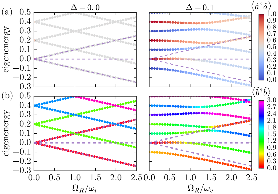
Figure 6.2: (a) Photonic components in the eigenspectrum of the HTC model for a single molecule as a function of the ratio between Rabi frequency \Omega_R and vibrational frequency \omega_v . (b) Vibrational component. Dashed purple lines indicate the upper and lower vibration-free polariton energies. The energy origin is set at \omega_e = \omega_O = 0 .
