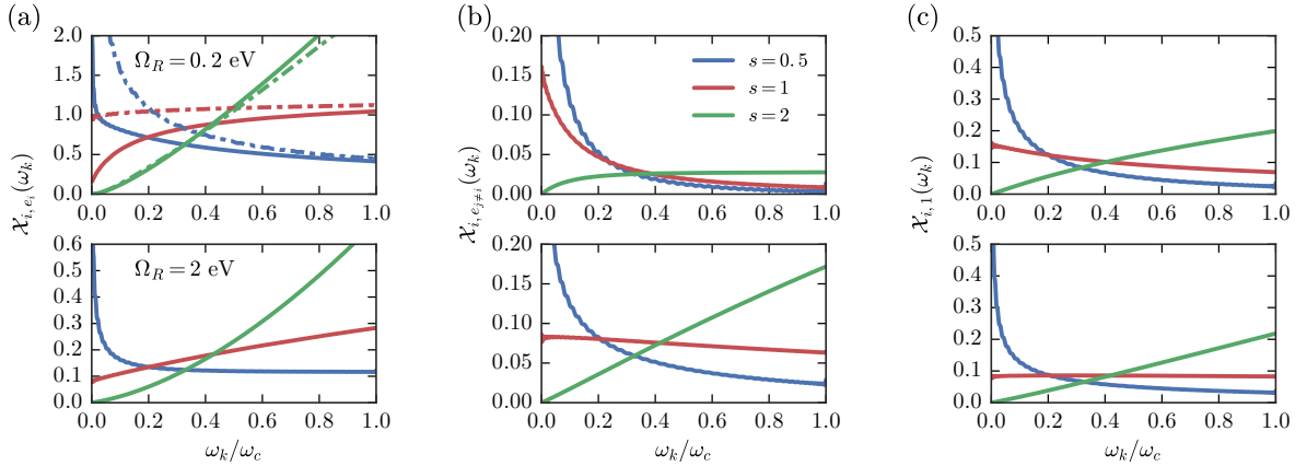
Figure 6.8: Absolute displacement spectrum of the phononic modes for a molecule i , projected on (a) the electronic state of the excited molecule, the electronic state of the unexcited molecule (b) and the cavity photon (c). In these panels we considered \Omega_v = 0.2 eV and N = 5 .
