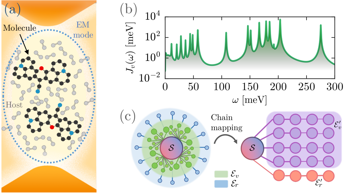
Figure 7.1: (a) Sketch of a molecular ensemble interacting with a confined EM resonance (dashed region) and with the host environment (grey circles). (b) Vibrational spectral density for Rhodamine 800 molecule. (c) Scheme illustrating the mapping of the vibrational modes yielding the multi-chain Hamiltonian used in the simulations.
