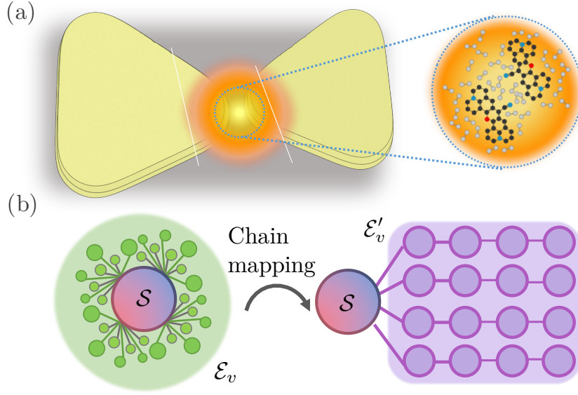
Figure 6.1: (a) Sketch of a molecular ensemble interacting with a confined EM resonance (dashed region) and with the host environment (grey circles). (b) Scheme illustrating the mapping of the vibrational modes yielding the multi-chain Hamiltonian used in the simulations, where the excitons interact with collective reaction coordinates in the molecules.
