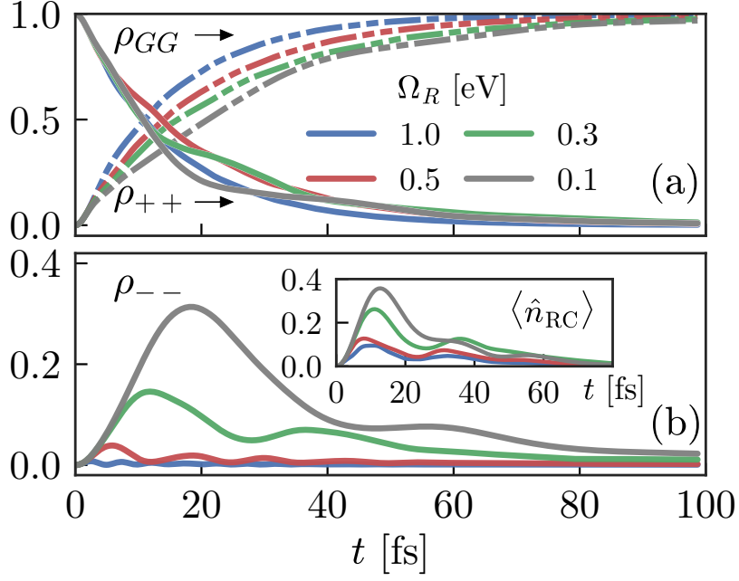
Figure 7.2: Dynamics of reduced density matrix populations for a single molecule as a function of the Rabi frequency \Omega_R , including (a) vacuum and upper polariton states and (b) the lower polariton. The inset in (b) shows the occupation of the collective reaction coordinate in the vibrational environment.
