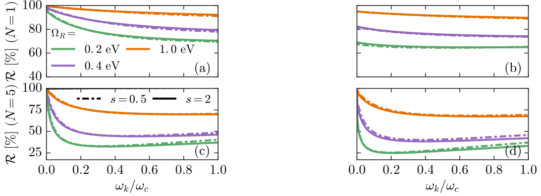
Figure 6.9: Ratio \mathcal{R} between displacement at \Omega'_R = 2 eV and lower Rabi frequency displacements, for the SBM at N = 1 (a),(b), and N = 5 (c),(d). The case \Delta = 0.01 eV is shown in left panel ((a),(c)) panel while \Delta = 0.1 eV is depicted in the right ((b),(d)). Two distant power laws s = 0.5 and s = 2 are shown.
