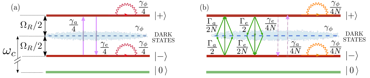
Figure 3.3: Illustration of the different decay and dephasing mechanisms that emerge from our modelling for the two dephasing scenarios: common bath (a) or independent baths (b). The arrows indicate decay processes while wavy lines represent elastic events that produce dephasing. The fuzzy halo around the dark states indicates excitation transfer and dephasing acting within this manifold.
