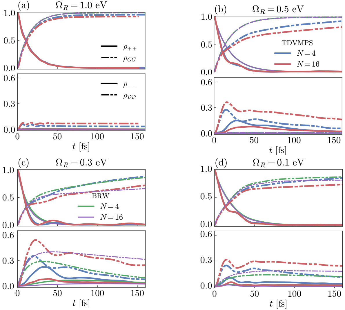
Figure 7.4: Population dynamics for N > 1 at different Rabi frequencies (shown in titles). The occupations \rho_{GG} , \rho_{++} are displayed in the upper panels, while \rho_{--} , \rho_{DD} is shown in the lower ones, with distinctive line styles. Colours blue and red depict cases of N = 4 and N = 16 while green and purple correspond to the Markovian limit calculated as described in the text.
