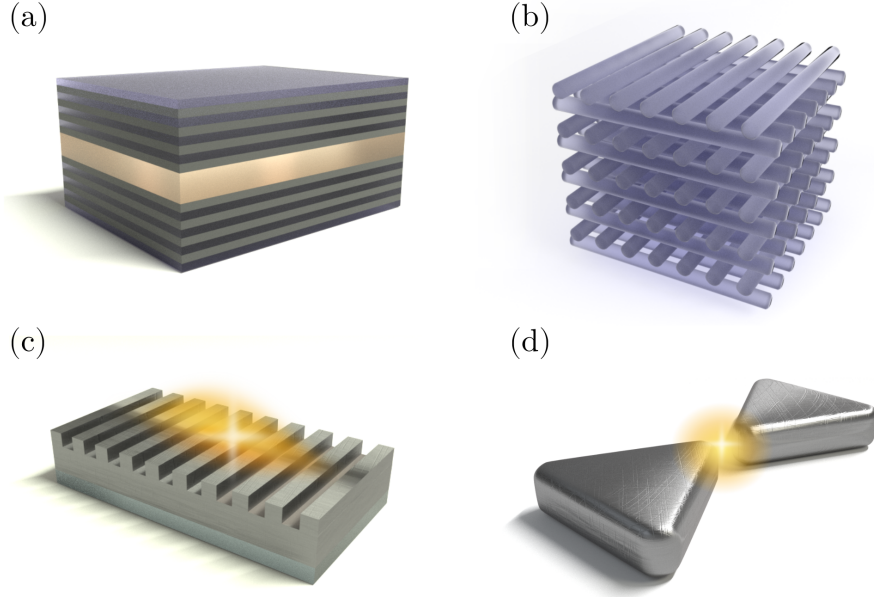
Figure 1.2: Conceptual depictions of some model structures employed to confine light. (a) Fabry–Perot microcavity based on distributed Bragg reflectors. (b) Three-dimensional photonic crystal. (c) Surface plasmon polaritons on a structured metallic surface. (d) Bow-tie nanoantenna hosting a strongly localized surface plasmon resonance.
