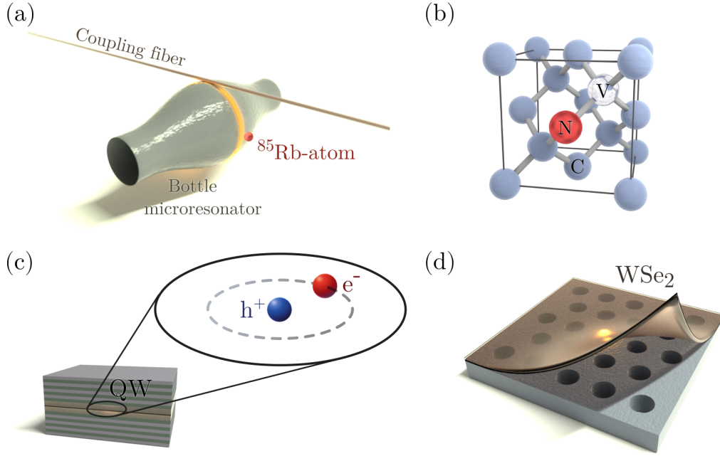
Figure 1.3: Examples of different quantum emitters. (a) A rubidium atom strongly coupled to a whispering-gallery-mode microresonator, itself coupled to an optical waveguide, as in reference [60]. (b) Simplified atomistic structure of a nitrogen-vacancy center in diamond. (c) DBR microcavity with an inorganic semiconductor quantum well in the center hosting Wannier-Mott excitons (schematically depicted in zoom). (d) Monolayer of WSe 2 (a transition metal dichalcogenide) coupled to a photonic crystal cavity, as in reference [61].
