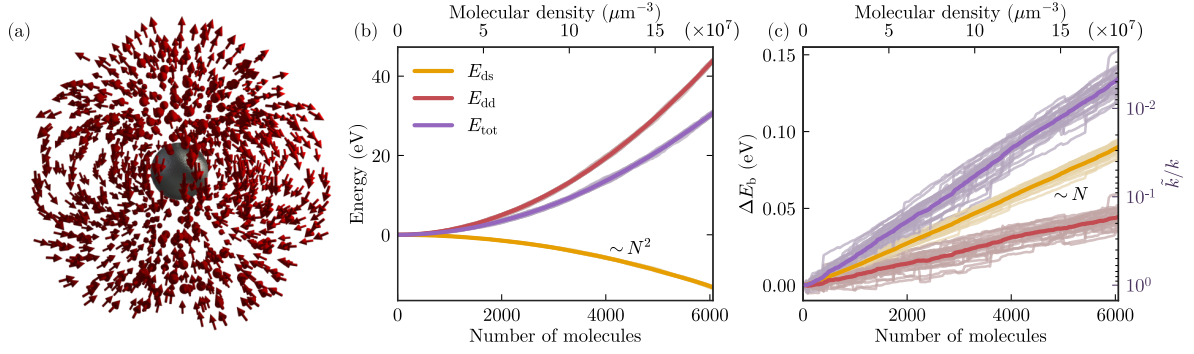
Figure 6.9: (a) Sketch of the model system of a collection of molecules distributed around a metal nanosphere with a diameter of 8 nm. The molecules are placed randomly at distances from 1 nm to 16 nm to the surface of the sphere, with the (permanent) dipoles aligned along the direction of the field of the sphere’s z -oriented dipole mode. (b) Energy due to the dipole-sphere ( E_{ds} ) and dipole-dipole ( E_{dd} ) interactions in the system within perturbation theory as a function of number of molecules N , as well as their sum ( E_{tot} ). (c) Change in energy barrier and corresponding change in reaction rate at room temperature for the most strongly coupled molecule, also resolved into contributions from dipole-sphere and dipole-dipole interactions. In both panels (b) and (c), the slightly transparent lines correspond to different random realizations of the system, with the averages in solid lines.
