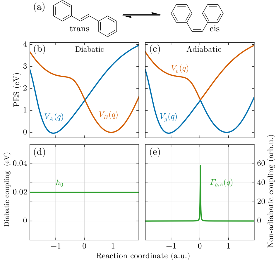
Figure 5.1: (a) Sketch of the cis-trans isomerization reaction of stilbene. (b) Diabatic and (c) adiabatic PES for the model molecule. (d) Constant coupling between the diabatic surfaces. (e) Nonadiabatic coupling at q \approx 0 between adiabatic surfaces V_g(q) and V_e(q) .
