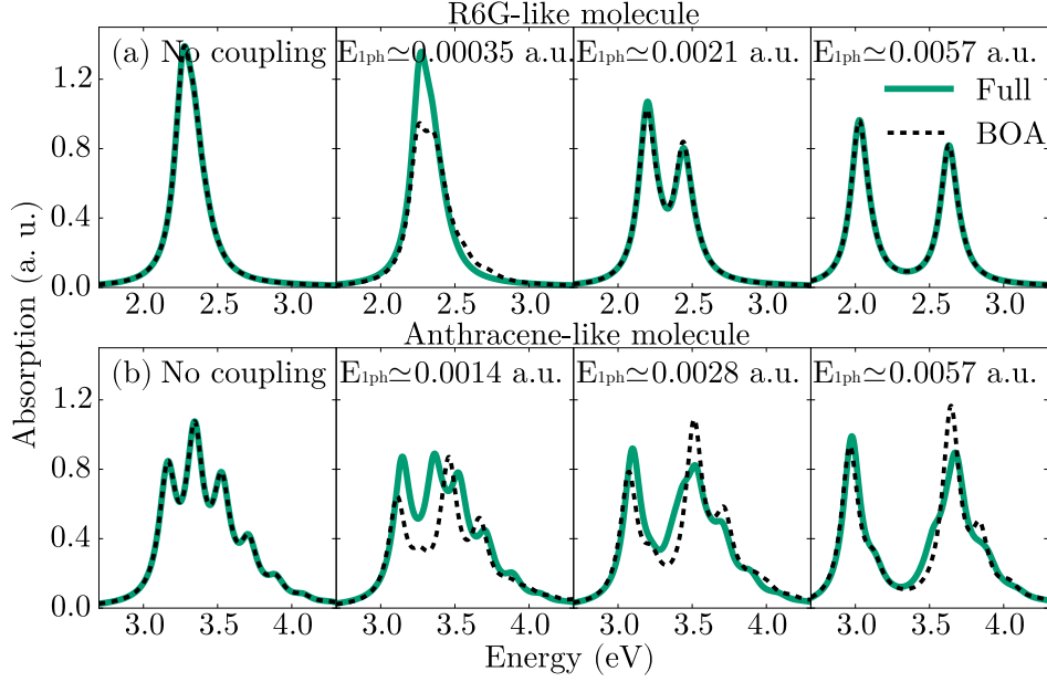
Figure 3.8: Absorption cross section of two molecules driven coherently, calculated using the full Hamiltonian without approximation (solid green lines) and within the BOA (dashed black lines). Results are shown for the (a) R6G-like and (b) anthracene-like model molecules, for several values of the coupling strength E_{1ph} . The values of E_{1ph} are scaled by 1/\sqrt{2} with respect to the single-molecule case (Fig. 3.4a and Fig. 3.5a) in order to obtain the same total Rabi frequency \Omega_R .
