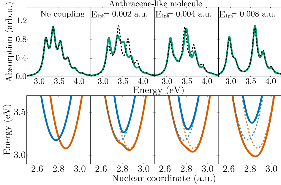
Figure 3.5: Top row: Absorption cross sections of a single anthracenelike model molecule, calculated using the full Hamiltonian without approximation (solid green lines) and within the BOA (dashed black lines) for several values of the coupling strength. Bottom row: Corresponding single-molecule PES in the single-excitation subspace in strong coupling (solid lines) and uncoupled (dashed lines).
