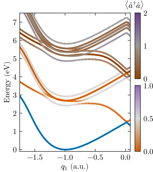
Figure 5.6: PoPES up to the two-excitation subspace for the treated model molecule, for N = 50 molecules, photonic mode frequency \omega_c = 2.65 eV, and (collective) Rabi frequency fixed to \Omega_C = 0.5 eV. The two color scales indicate the photon fraction in the single- and two-excitation subspace, respectively.
