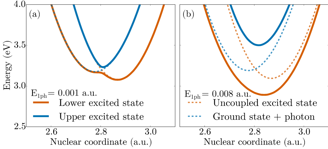
Figure 3.3: Strongly coupled electronic PES (solid lines) in the singly excited subspace, for the anthracene-like molecule for (a) E_{1\text{ph}} = 0.001 a.u. and (b) E_{1\text{ph}} = 0.008 a.u.. The dashed lines show the corresponding uncoupled states: A molecule in the first excited state, V_e(R) , and a molecule in the ground state with one photon present, V_g(R) + \omega_c .
