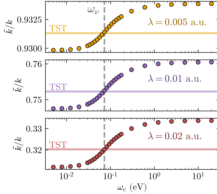
Figure 6.6: Ratio between on- ( \tilde{k} ) and off-cavity ( k ) rates vs the cavity frequency for three different values of the coupling strength. We increase the density of points close to the vibrational frequency of the molecule \omega_\nu \approx 72.6 meV in order to explore potential resonance effects.
