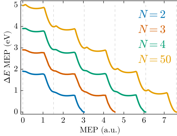
Figure 5.11: Energy profile along the minimum energy paths for collections of 2, 3, 4 and 50 molecules. For N = 50 , only the first five steps are shown explicitly. Thin dashed lines indicate the approximate location along the path where one molecule stops moving and the next one starts.
