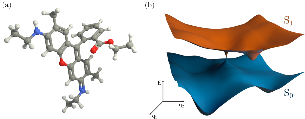
Figure 1.4: Complexity of organic molecules. (a) Depiction of a rhodamine 6G molecule, commonly used for achieving organic polaritons. (b) Conceptual example of energy dependence with nuclear coordinates q_1 and q_2 of the first two electronic states ( S_0 and S_1 ) of an organic molecule. These, in general, multidimensional hypersurfaces are known as potential energy surfaces. Typical energy landscapes have a dependence on many nuclear degrees of freedom and present multiple electronic states.
