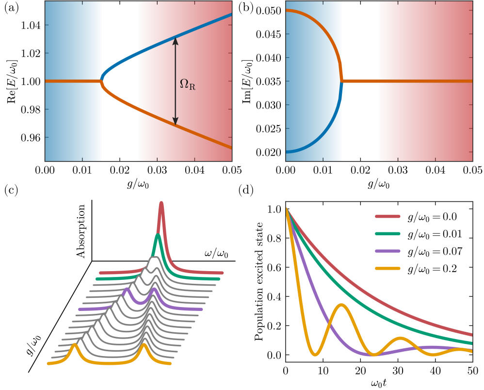
Figure 2.4: Simple representation of the weak and strong coupling regimes. (a) Real part of the eigenenergies and (b) decay rates of the eigenstates (polaritons) of the Hamiltonian as a function of the coupling strength. (c) View of the energy splitting in the absorption spectrum for different values of the coupling strength. (d) Population dynamics for the stated initiated in the excited emitter state |e\rangle . The decay rates are \gamma/\omega_0 = 0.04 and \kappa/\omega_0 = 0.1 .
