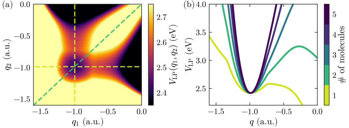
Figure 5.3: Many-molecule potential energy surfaces under strong coupling. (a) Lower polariton PES for N = 50 molecules, under motion of molecules 1 and 2, with all others held in the equilibrium position q_0 . (b) Energy reaction path corresponding to simultaneous motion of several molecules. In both panels, the photonic mode frequency is \omega_c = 2.65 eV, while the (collective) Rabi frequency is fixed to \Omega_C = \sqrt{N}\Omega_R = 0.5 eV.
