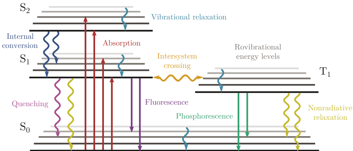
Figure 1.5: Jablonski diagram depicting the possible processes typically present in organic molecules. Electronic states are denoted by their total spin (S for singlet and T for triplet) and are schematically represented by their rovibrational structure. Straight arrows represent events in which single optical photons are transferred, while wavy arrows depict processes in which energy is transmitted in the form of nuclear motion of the molecule and/or its environment.
