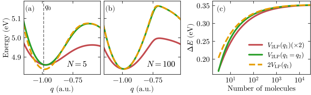
Figure 5.7: (a,b) Comparison of the PoPES in the double-excitation subspace for motion of one molecule (red line) and two molecules (green line), and twice the lower PoPES in the single-excitation subspace for motion of one molecule (orange dashed line), for N = 5 and N = 100 coupled molecules, respectively. (c) Dependence of the energy barrier for double photoisomerization with the number of molecules for the reaction paths corresponding to the PoPES in (a,b).
