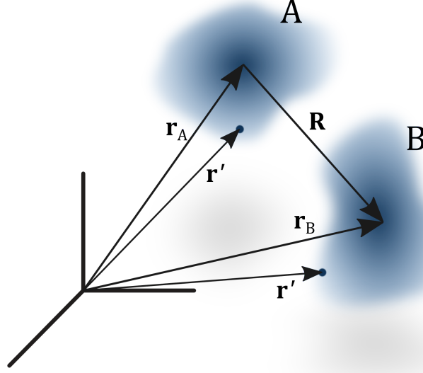
Figure 2.1: Scheme of two interacting charge distributions in space.
