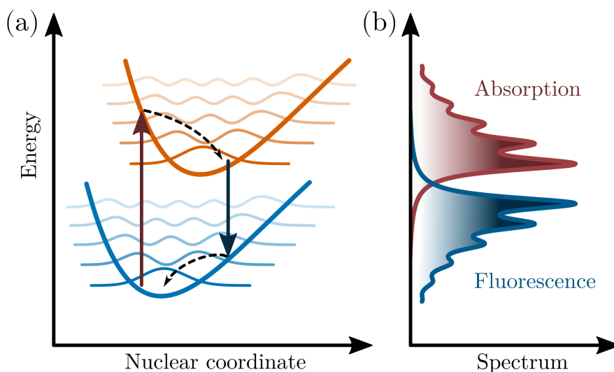
Figure 2.3: (a) Typical simplified picture of the energy landscape of an organic molecule with different processes represented: absorption (dark red arrow), emission (dark blue arrow), and nuclear relaxation (dashed black arrows). (b) Corresponding absorption and emission (fluorescence) spectra for this model system.
