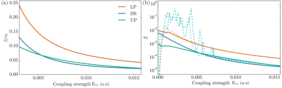
Figure 3.9: (a) Coupling between nuclear motion in different molecules for the lower (LP) and upper polariton (UP) and dark-state (DS) PES. Results are shown as the ratio \beta/\alpha between the prefactors of the offdiagonal R_1 R_2 and diagonal R_i^2 terms in Eq. (3.16), for the R6G-like model molecule. (b) Mutual information in the nuclear probability distribution for two different states. The solid lines correspond to the vibrational ground states of the coupled PES as predicted by Eq. (3.19) using the values of \beta/\alpha shown in (a), while the dashed lines correspond to the steady state under driving of a single molecule as defined in Eq. (3.17).
