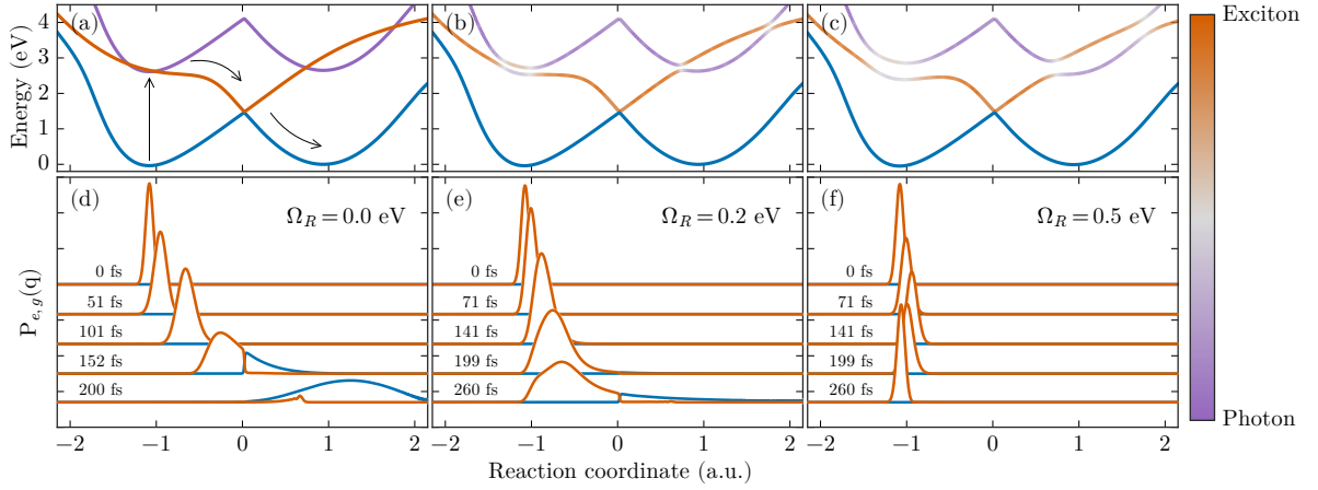
Figure 5.2: Suppression of photoisomerization under strong coupling for a single molecule. (a-c) Ground (blue) and excited (purple-orange color scale) potential energy surfaces of the model molecule coupled to a quantized light mode ( \omega_c = 2.65 eV), with the light-matter coupling strength \Omega_R increasing from (a) to (c). The continuous color scale encodes the nature of the hybridized excited PES. (d-f) Time propagation of the nuclear wavepacket after sudden excitation to the lowest excited PES (lower polariton for \Omega_R > 0 ), shown separately for the parts in the lower polariton surface (orange) and the ground state surface (blue) reached through the nonadiabatic transition at q = 0 . Contributions in the upper polariton surface are negligible and not shown.
