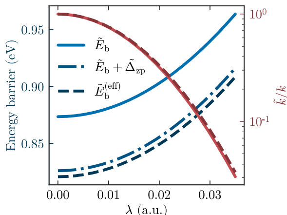
Figure 6.4: Energy barrier and rates ratio vs coupling strength for the case of a CBOA calculation (full lines) and for the effective energy barrier fitted from exact quantum rate calculations (dashed lines).
