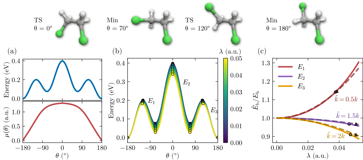
Figure 6.8: Top: Different configurations along the internal rotation of 1,2-dichloroethane. (a) Energy landscape and dipole moment of the molecule. (b) Modified energy path for minimum q for different coupling strengths. The energy barriers of the bare molecule are defined as E_1 = V(120^\circ) - V(70^\circ) , E_2 = V(0^\circ) - V(70^\circ) , and E_3 = V(120^\circ) - V(180^\circ) . (c) Relative modification of the energy barriers depending on the coupling strength for the full calculation (full lines, circles) and for perturbation theory (dashed lines, triangles). The marked points indicate relevant changes in the rate.
