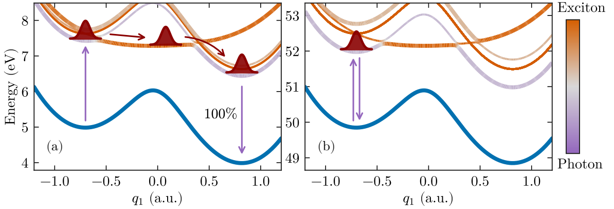
Figure 5.9: Potential energy surfaces of a system with one light mode and (a) N = 5 molecules in the strong coupling regime with Rabi frequency \Omega_R = 0.3 eV and photon energy \omega_c = 2.55 eV, and (b) N = 50 molecules with Rabi frequency \Omega_R = 0.75 eV and photon energy \omega_c = 2.4 eV. All molecules but one are fixed at the initial position ( q_1 = q_{\text{ms}} \approx -0.7 a.u.). The color scale represents the cavity mode fraction of the excited states, going from pure photon (purple) to pure exciton (orange).
