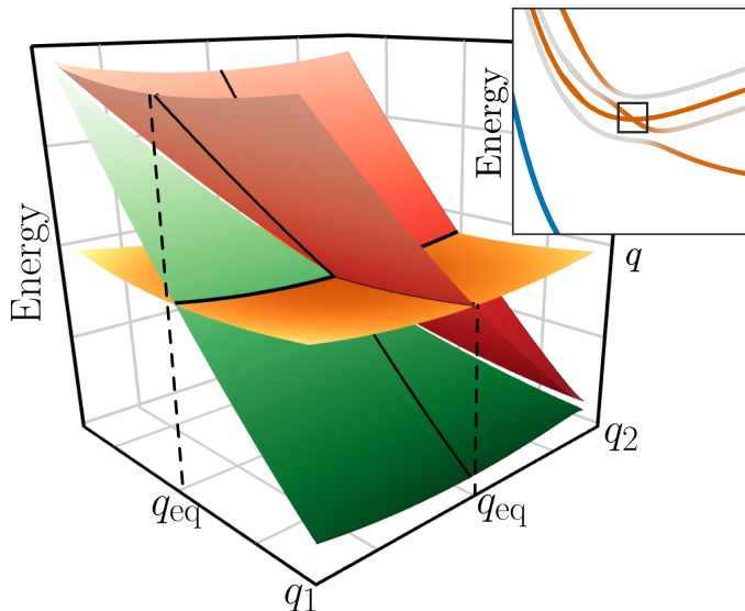
Figure 4.3: Zoom on the collective light-induced conical intersection between dark-state PoPESs under motion of two molecules.
