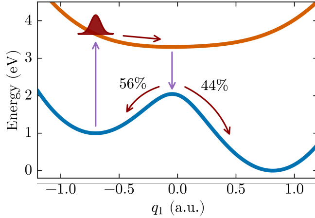
Figure 5.8: Potential energy surfaces of a molecule presenting a general photoisomerization reaction where one isomer has higher energy than the other, both of them with roughly equal reaction quantum yield after absorption of a photon.
