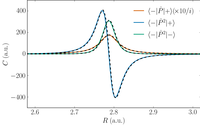
Figure 3.6: Nonadiabatic correction terms C that couple the “lower polariton” and “upper polariton” PES for a single anthracene-like model molecule for a coupling strength of E_{\text{1ph}} = 0.002 a.u.. Solid colored lines: results from a full numerical calculation. Dashed black lines: results from the model Eq. (3.9). Note that while all results are given in atomic units, the units of the \hat{P} and \hat{P}^2 terms are not identical, and thus not directly comparable.
