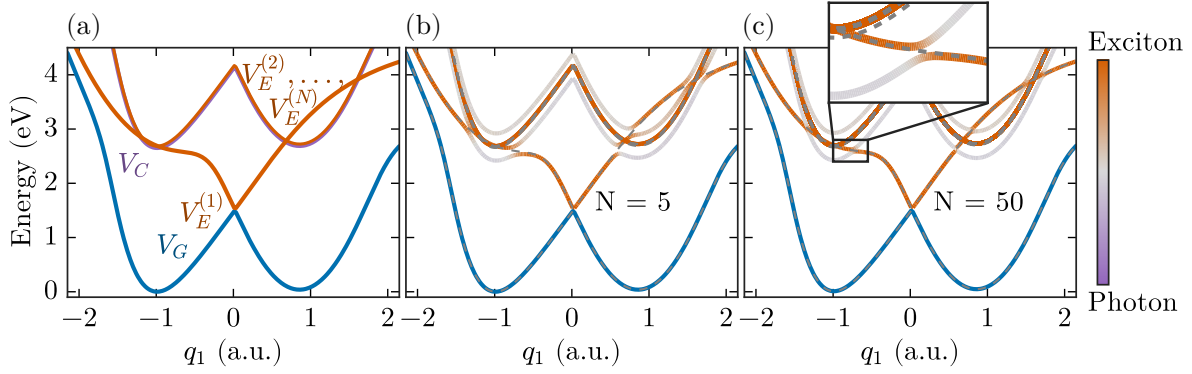
Figure 5.4: Many-molecule potential energy surfaces under strong coupling. (a-c) All potential energy surfaces under motion of only molecule 1, for no light-matter coupling (a), and under strong coupling for N = 5 (b) and N = 50 (c) molecules. In all panels, the photonic mode frequency is \omega_c = 2.65 eV, while the (collective) Rabi frequency is fixed to \Omega_C = \sqrt{N}\Omega_R = 0.5 eV.
