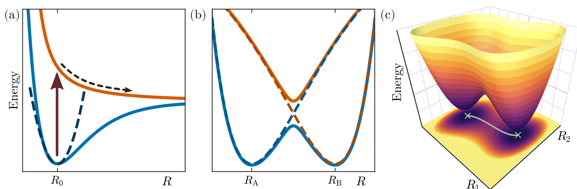
Figure 2.2: Some common conceptual energy landscapes in chemistry. (a) Bond dissociation picture. (b) Isomerization scenario between two stable configurations R_A and R_B . (c) Two-dimensional ground state surface with two stable configurations connected by a minimum energy path (light gray line).
