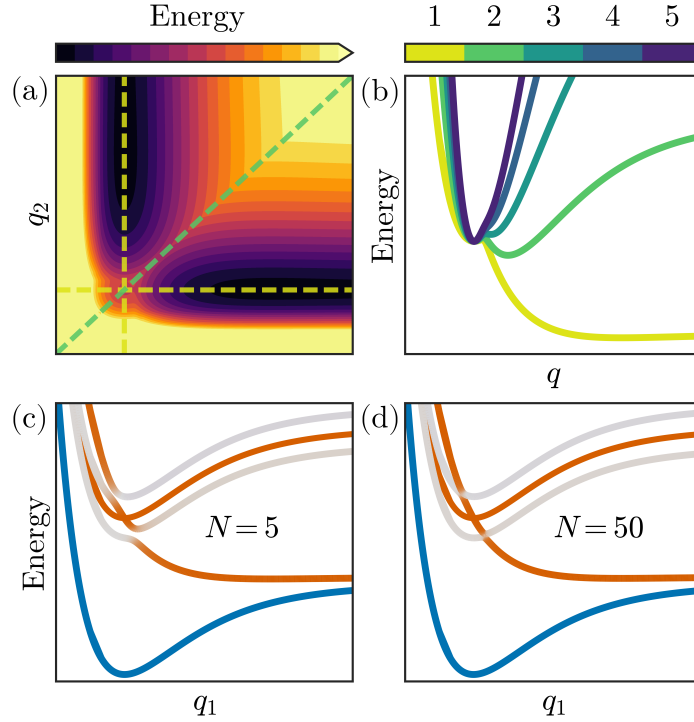
Figure 4.2: Collective energy landscape in the single-excitation subspace. (a) Lowest excited two-dimension PoPES for motion of two molecules of N = 50 molecules. (b) Lowest excited PoPES for correlated simultaneous motion of n = 1, \dots, 5 molecules (for the N - n remaining molecules in the equilibrium position, with N = 50 ). (c,d) Full PoPES for motion of one molecule for the case of (c) N = 5 molecules and (d) N = 50 molecules, with identical color code to those in Fig. 4.1.
