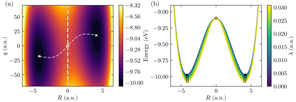
Figure 6.3: (a) Two-dimensional ground-state PES in the cavity Born–Oppenheimer approximation for the Shin–Metiu model for \lambda = 0.02 a.u. and \omega_c = 72.6 meV. At R = 0 we show the dividing surface used to compute the reaction flux from reactant to product states. The gray dashed line curve corresponds to the energy path along q_m(R) , i.e., the minimum in q . (b) Value of the energy path \tilde{V}_g(\mathbf{R}, q_m) for different values of the Rabi frequency, which is related to the coupling strength through \Omega_R = \lambda \mu'_g(R_0) , where the dipole derivative is evaluated at the minimum.
