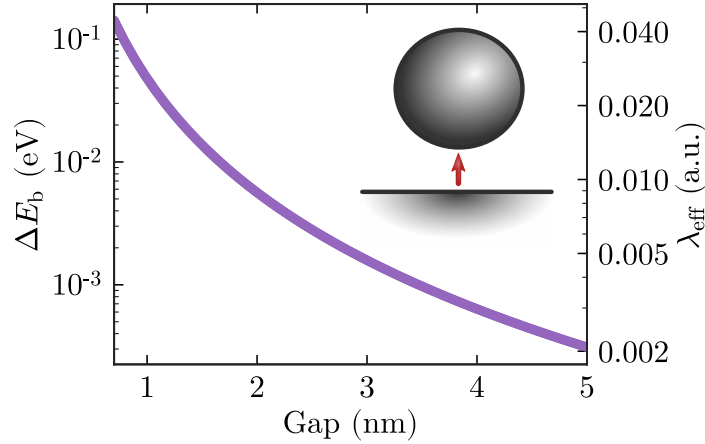
Figure 6.7: Change of the energy barrier for the Shin-Metiu model inside a nanoparticle-on-mirror cavity as a function of gap size. The right y -axis shows the corresponding values of the effective single-molecule coupling strength \lambda_{\text{eff}} = \sqrt{\sum_k \lambda_k^2} . Inset: Illustration of nanoparticle-on-mirror cavity geometry, with a single molecule placed in the nanogap between a planar metallic surface and a small metallic nanoparticle of radius R = 20 nm.
