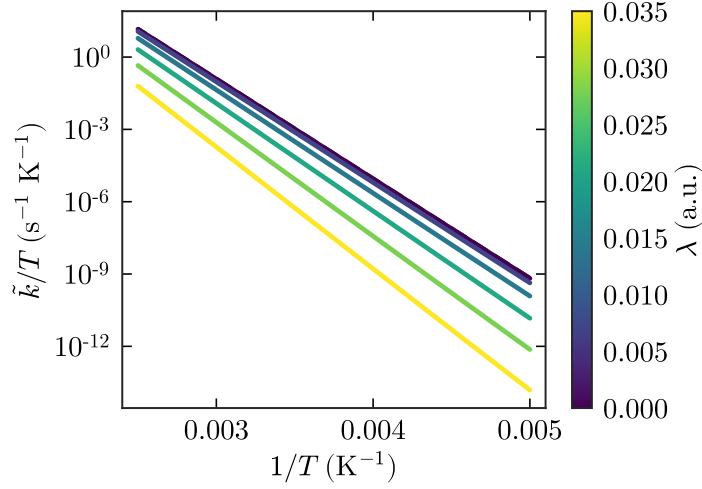
Figure 6.2: Arrhenius plot for the rate dependence with temperature in the hybrid system for several light-matter coupling values. See main text for details.
