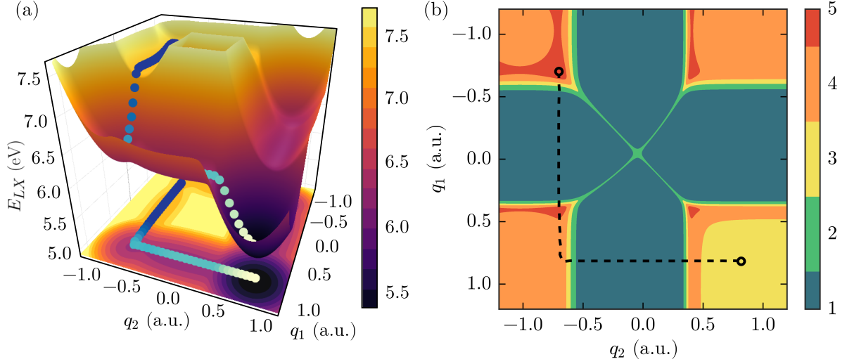
Figure 5.10: (a) Lowest-energy excited state PES for 2 moving molecules in a 5-molecule ensemble. The minimum energy path (blue to white dots) connects the initial excited region with the final configuration of the two molecules. (b) Participation ratio map of the lowest-energy excited state, indicating over how many molecules the state is delocalized. The MEP is indicated by a dashed black line.
