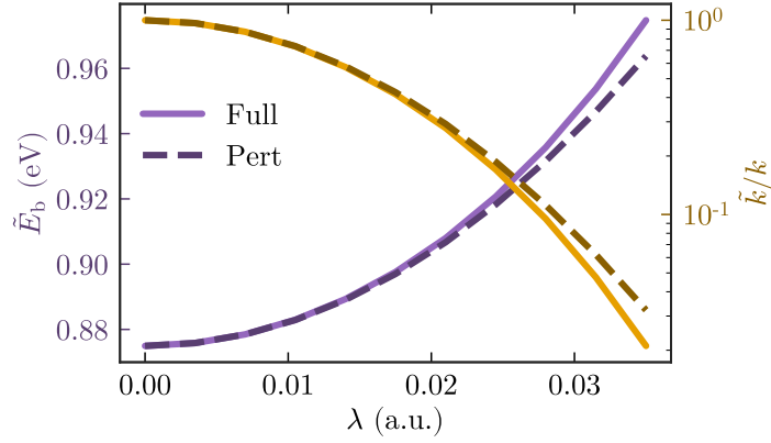
Figure 6.5: Cavity Born–Oppenheimer energy barrier (purple) and relative change of reaction rates (yellow) for the Shin–Metiu model inside a cavity, calculated to all orders in the light-matter coupling strength \lambda (solid lines), and up to second order in perturbation theory (dashed lines).
