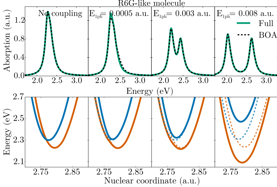
Figure 3.4: Top row: Absorption cross sections of a single R6G-like model molecule, calculated using the full Hamiltonian without approximation (solid green lines) and within the BOA (dashed black lines) for several values of the coupling strength. Bottom row: Corresponding single-molecule PES in the single-excitation subspace in strong coupling (solid lines) and uncoupled (dashed lines).
