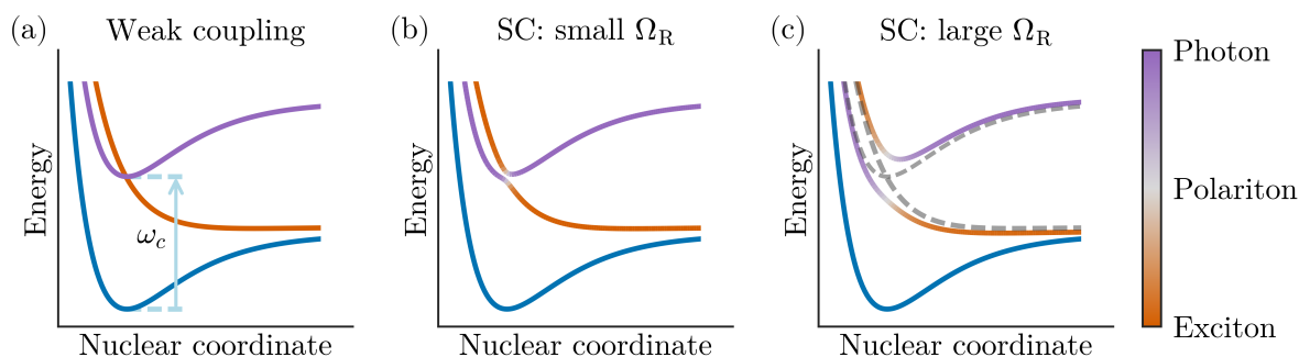
Figure 4.1: Conceptual potential energy surfaces for a single molecule describing a typical bound and dissociative energy landscape coupled to a light mode in (a) weak coupling and (b,c) strong coupling for different coupling strengths. The color represents the photonic fraction of the state from purely excitonic (orange) through polaritonic (light gray) to purely photonic (purple).
