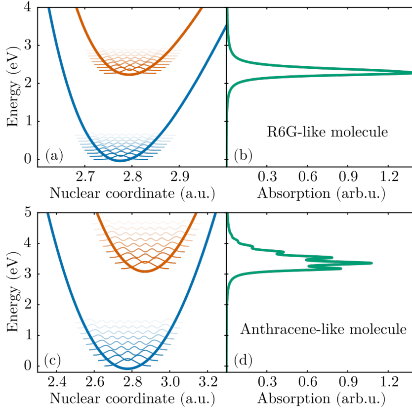
Figure 3.2: Bare-molecule potential energy surfaces of the two first electronic states in the BOA for (a) the rhodamine 6G-like model molecule and (c) the anthracene-like model molecule. The vibrational levels and associated nuclear probability densities are represented on top of the PES. (b) and (d): Absorption spectrum for the (b) R6G-like and (d) anthracene-like molecule in arbitrary units.
