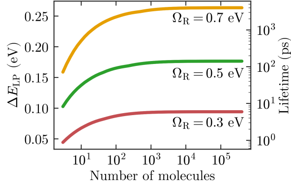
Figure 5.5: Energy barriers vs number of molecules for different values of Rabi splitting. The right axis shows the equivalent lifetime predicted through transition-state theory.
