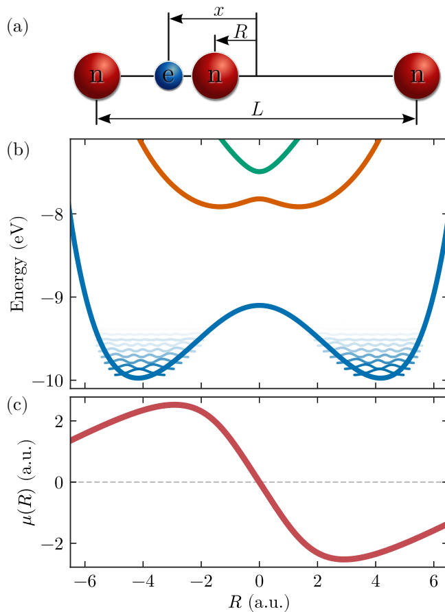
Figure 6.1: (a) Schematic representation of the Shin–Metiu model close to one of the equilibrium configurations. The two ions on both sides are fixed at a distance L , while the electron and the remaining ion can move freely in between. (b) Potential energy surfaces of the model with the vibrational levels and associated probability densities of the ground state (blue) represented. (c) Ground state dipole moment.
