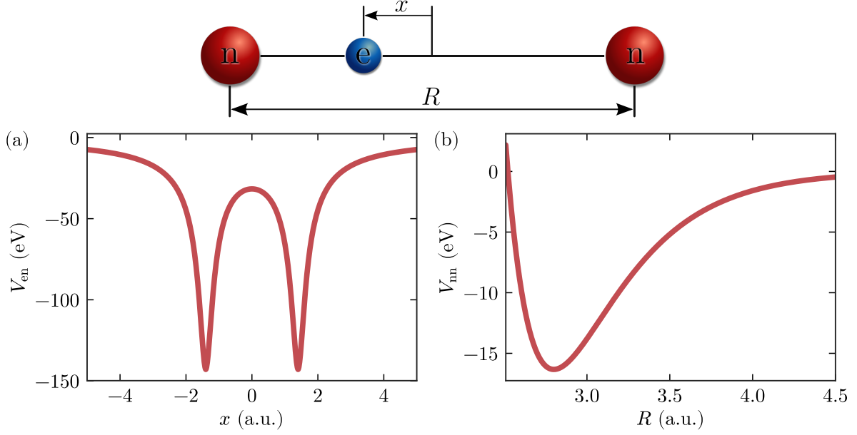
Figure 3.1: Top: schematic representation of our molecular model. Bottom: model potentials for (a) electron-nuclei and (b) nucleus-nucleus interactions.
