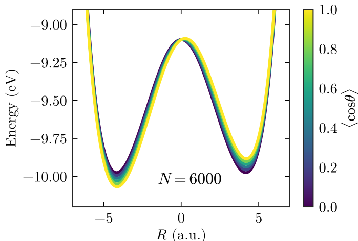
Figure 6.10: Alignment dependence of the cavity Born–Oppenheimer PES along the photonic minimum path q_m for the molecule in Fig. 6.9(c), with all other molecules fixed to the equilibrium position R_{\min} .
